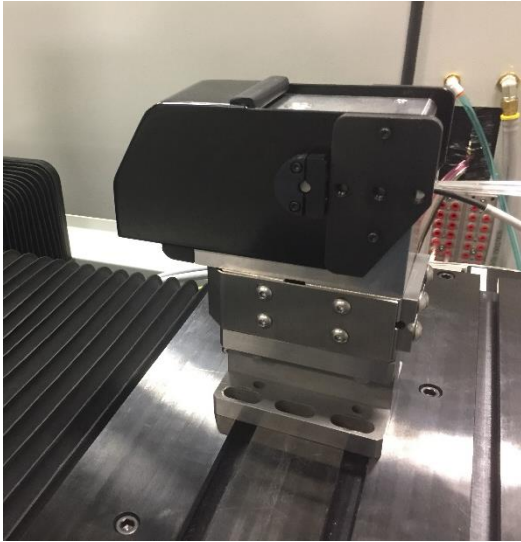
Part Centering Device (Shown with Protective Cover Closed)
