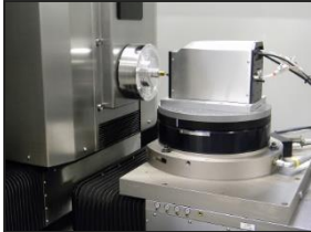
Fast Tool Servo on B-axis
